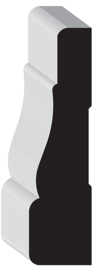
OW351 WM351 11/16" x 2-1/2" PFJP • SP 16' RL
