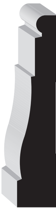
OW445 WM445 11/16" x 3-1/4" PFJP • SP • SO 15' RL
