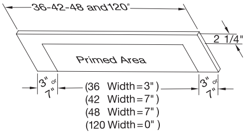
8110E GBR (Glue Block Ready) Primed Risers
